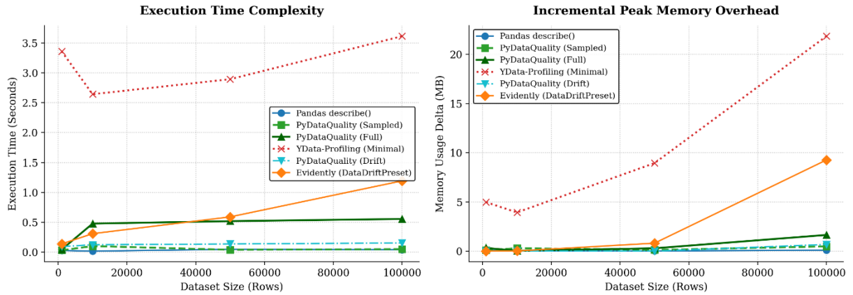
Figure 9: Performance benchmarking results across four dataset scales (1k–100k rows) comparing batch profiling tools and drift detection frameworks on execution time (left panel) and incremental peak memory overhead (right panel). PyDataQuality in sampled mode (light green) maintains near-constant complexity. YData-Profiling (red) exhibits high fixed overhead across all scales. Full derivation of these results is in Section 5.1.2 and 5.1.3. (Note: Evidently AI is excluded from pure single-dataset profiling comparisons as it focuses heavily on comparative drift.)
