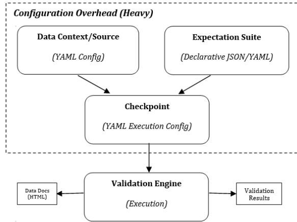
Figure 1: Illustration of the Great Expectations Configuration vs. Computation Workflow. While computationally robust, the operational burden is heavily skewed toward configuration, requiring developers to orchestrate multiple interconnected YAML and JSON artifacts (Data Contexts, Expectation Suites, and Checkpoints) before data validation can execute.
