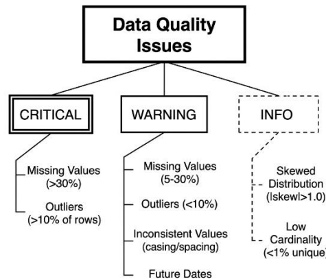
Figure 4: PyDataQuality Issue Taxonomy and Severity Classification.
