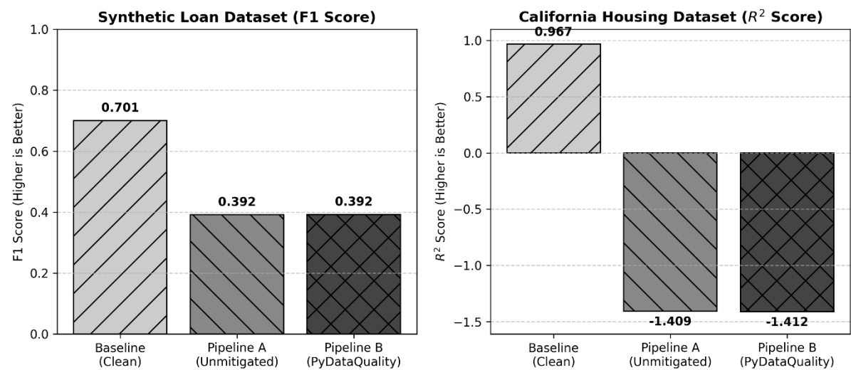
Figure 10: MLOps Pipeline Performance: Synthetic vs Real-World
